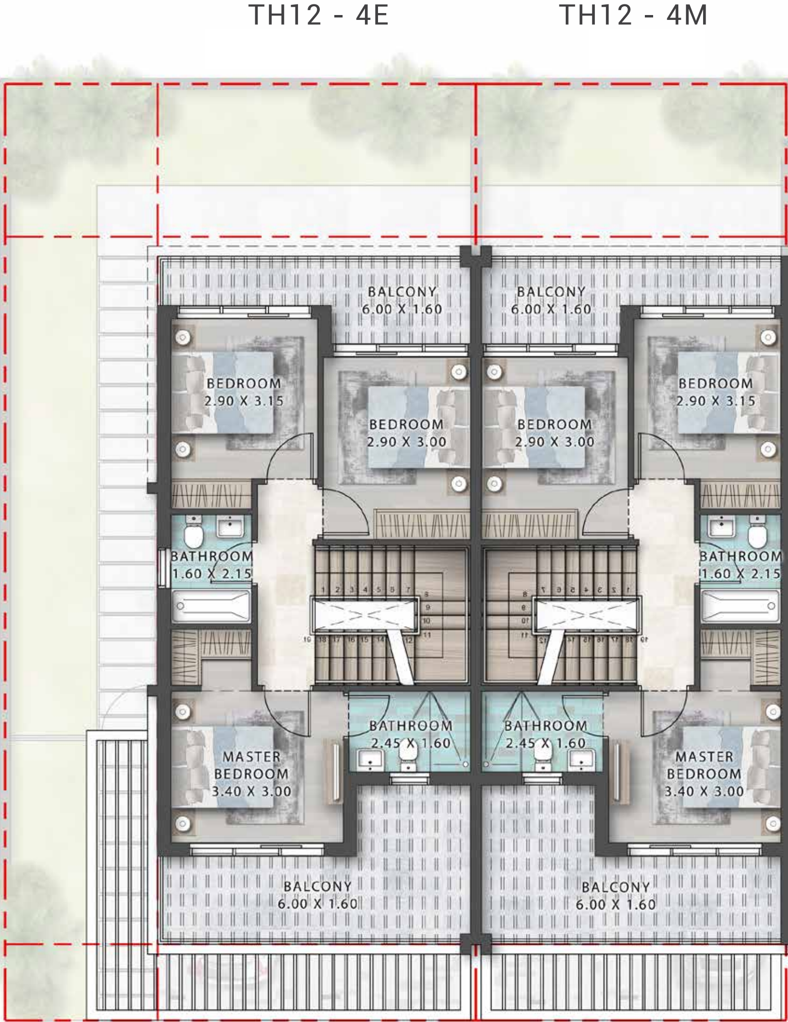
FIRST FLOOR
