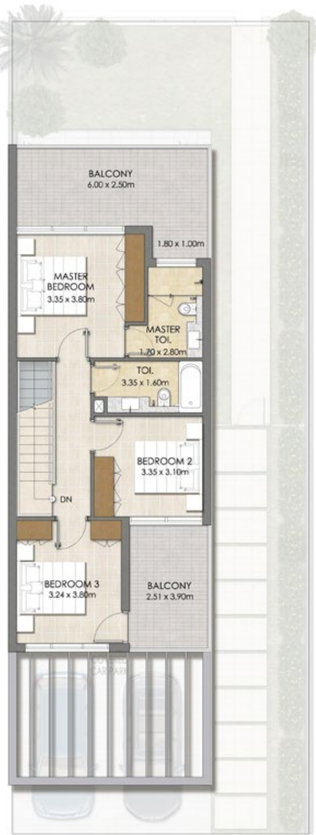
FIRST FLOOR
